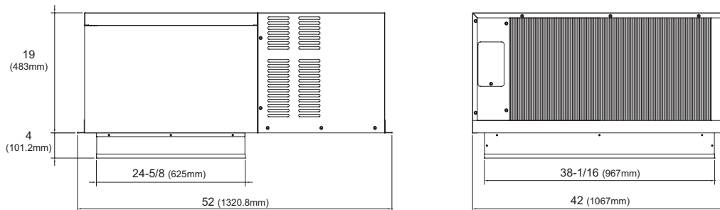
Figure C. Opening Size : 25" x 38 1/4"
